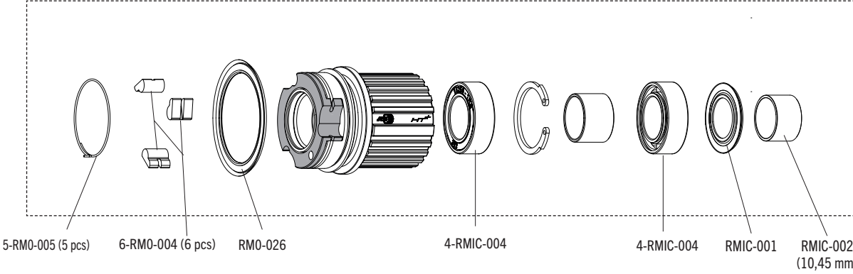
R0-127R (MICRO SPLINE 12 Ø33 mm ALU & STEEL)
